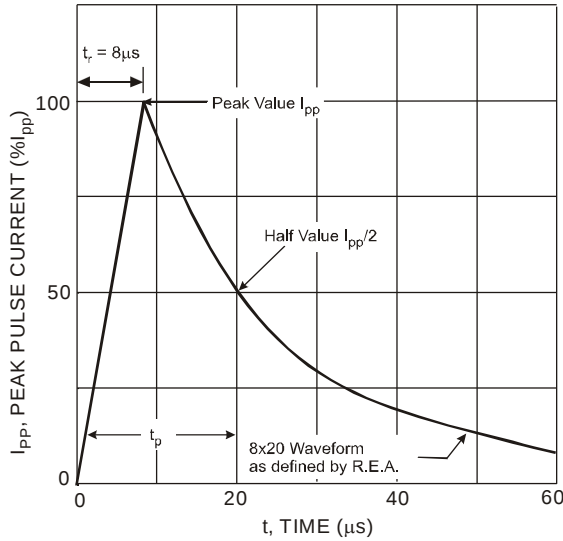
Figure 3 Typical 8 × 20 \mu s Pulse Waveform
