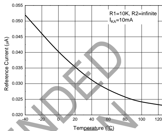
Reference Current vs. Ambient Temperature
