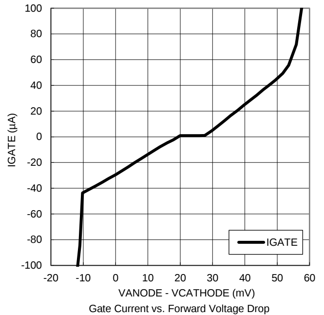
Gate Current vs. Forward Voltage Drop
