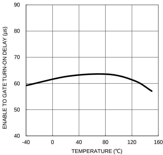
Enable to Gate Delay vs. Temperature
