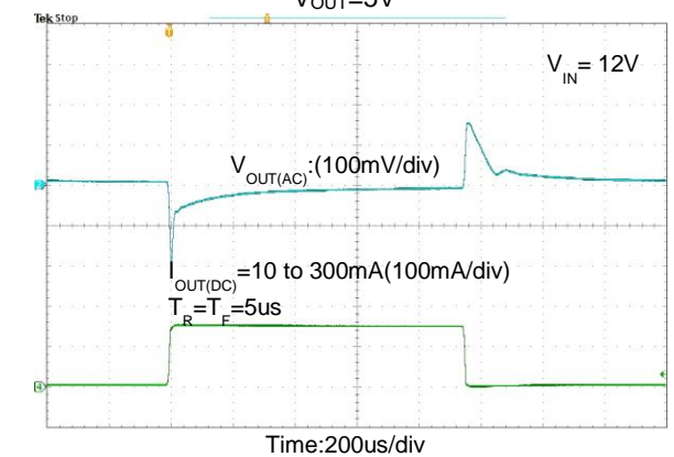
Load Transient Response V_{OUT} = 5\text{V}
