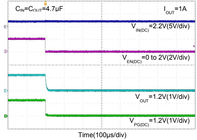
Enable Turn-Off Response V_{OUT}=1.2V
