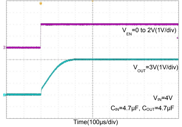
Start-up Time V_{OUT}=3V @ I_{OUT}=100mA
