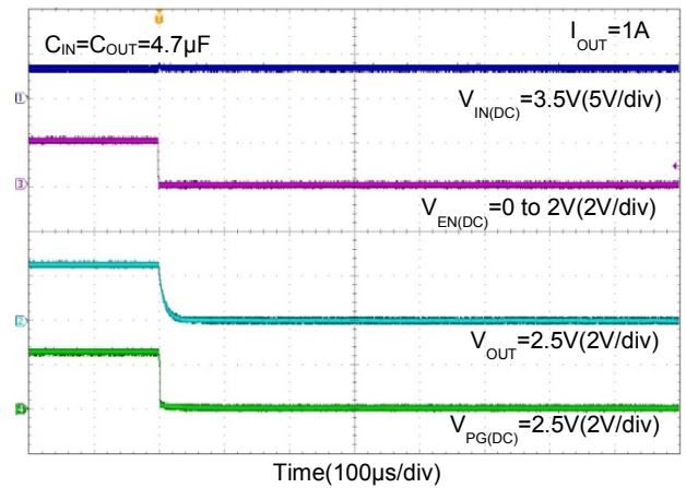
Enable Turn-Off Response V_{OUT}=2.5V
