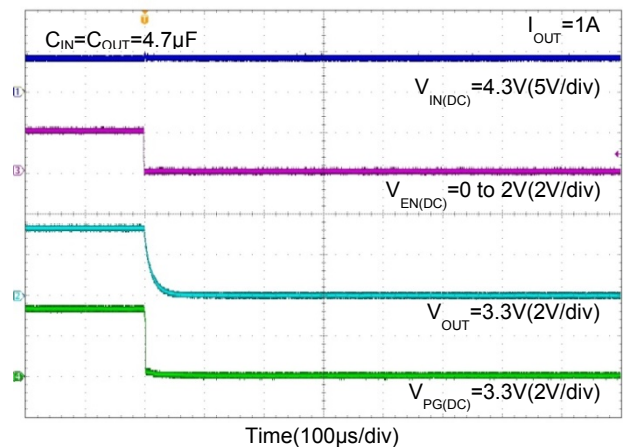
Enable Turn-Off Response V_{OUT}=3.3V
