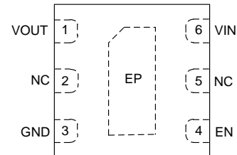
W-DFN2020-6 (SWP) (Type A1)
