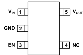
SOT25 (Type A1)
