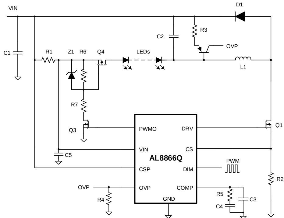
Figure 11 Buck LED Driver with PWM Dimming Operation
