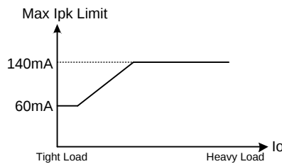
Figure 4. Maximum I_{PK} Limit Modulations with Output Load
