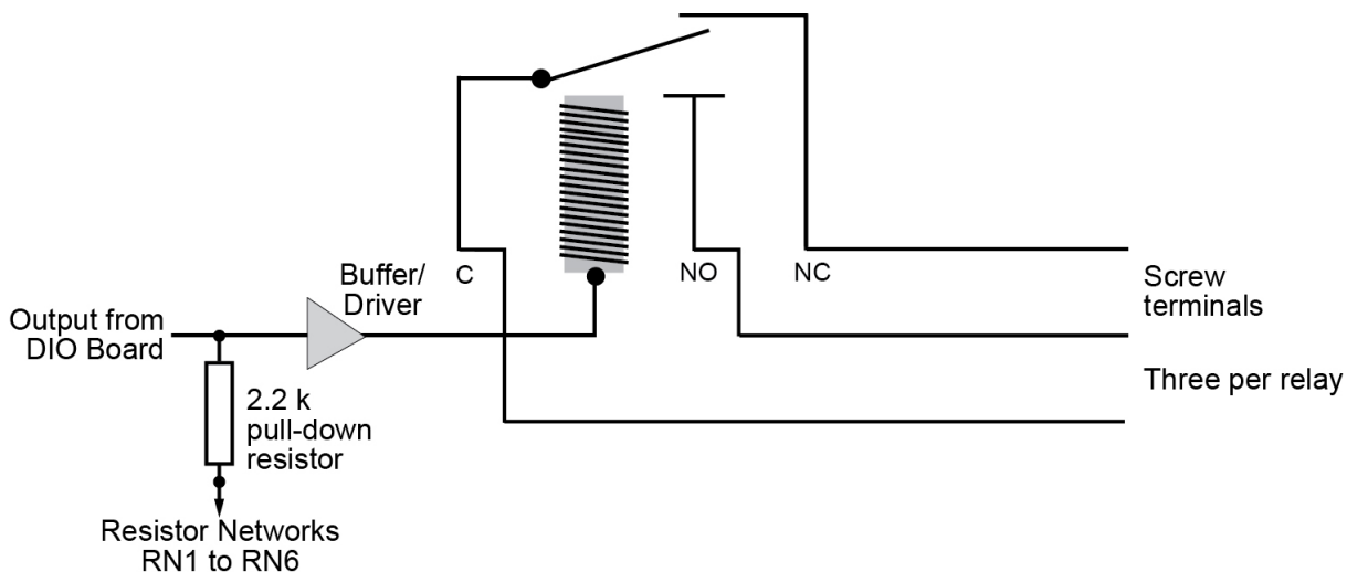
Figure 4. C/O-ERB48/C/O-SERB48 relay configuration
