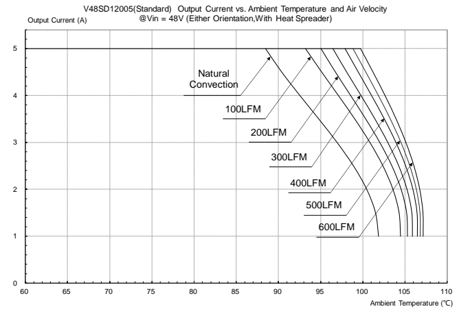
Figure 7: V48SD05012 Output current vs. ambient temperature and air velocity @ V_{in}=48V (Either Orientation, With Heat Spreader)
