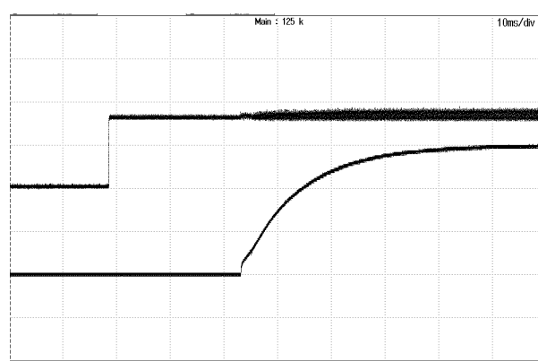
Figure 4: Turn-on transient at full load current (10ms/div). Top Trace: Vout; 5V/div; Bottom Trace: ON/OFF input: 2V/div.
