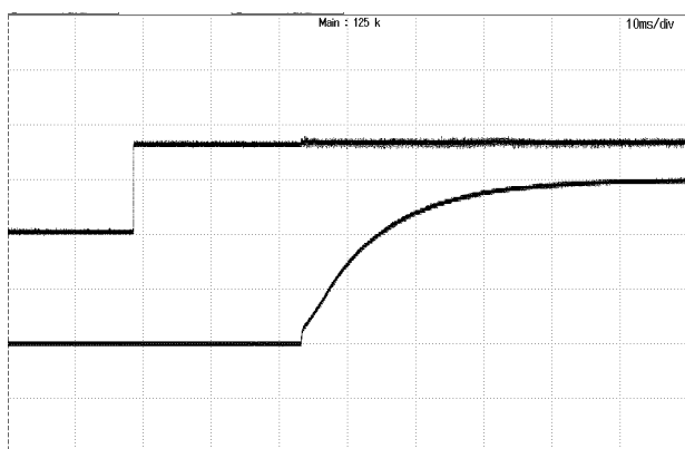
Figure 3: Turn-on transient at zero load current (10ms/div). Top Trace: Vout; 5V/div; Bottom Trace: ON/OFF input: 2V/div.
