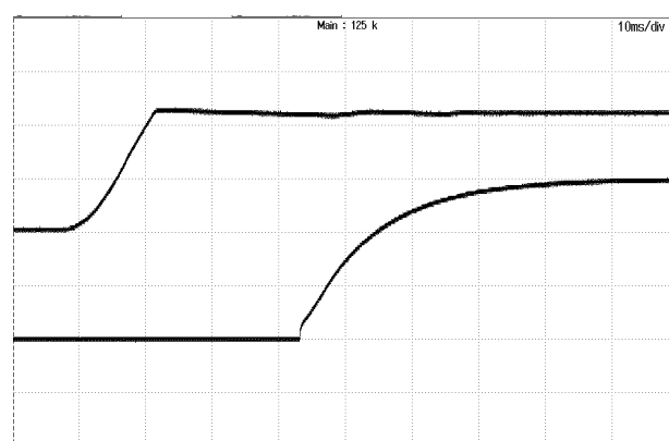
Figure 6: Turn-on transient at full load current (20ms/div). Top Trace: Vout; 5V/div; Bottom Trace: input voltage: 50V/div.
