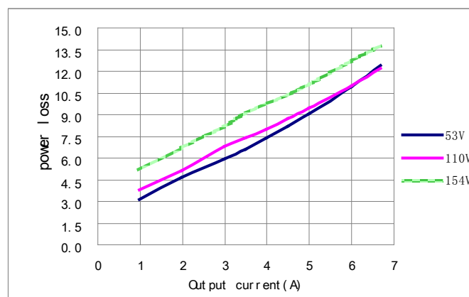
Figure 2: Power dissipation vs. load current for 66V, 110V, and 160V input voltage at 25°C.
