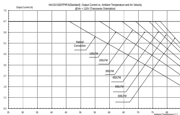
Figure 17: Output current vs. ambient temperature and air velocity @Vin=110V(Either Orientation, airflow from Vin- to Vin+,with heat spreader)
