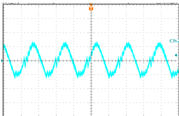
Figure 10: Output voltage ripple at nominal input voltage and max load current (10 mV/div, 2us/div) Bandwidth: 200 MHz.
