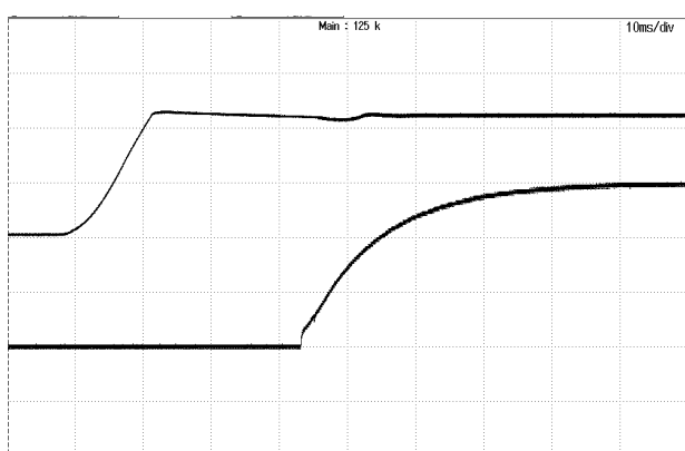
Figure 5: Turn-on transient at zero load current (20ms/div). Top Trace: Vout; 5V/div; Bottom Trace: input voltage: 50V/div.
