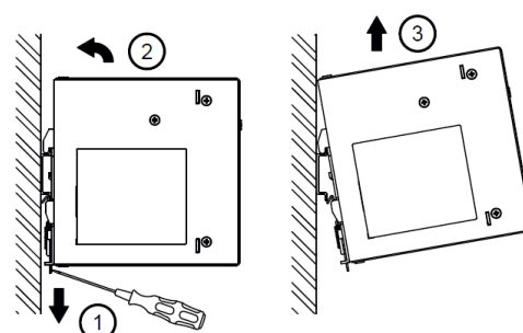
Fig. 3.2 Dismounting
