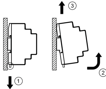
Fig. 2.2 Dismounting
