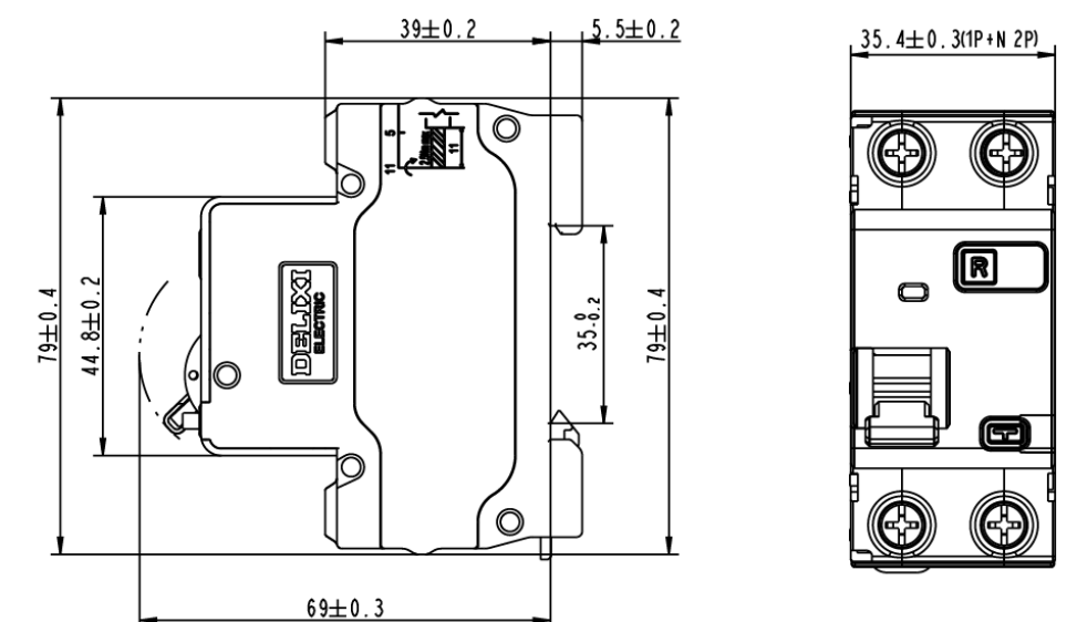
(1P+N, 2P)
