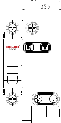
1P+N-63A
