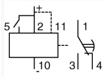
Timer 814 - 11-pin
