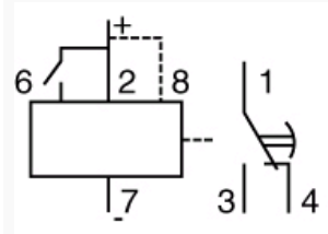
Timer 814 - 8-pin
