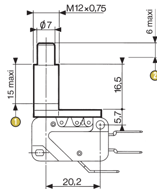
161L telescopic plunger
