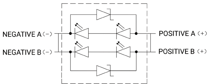
6-V Configuration
