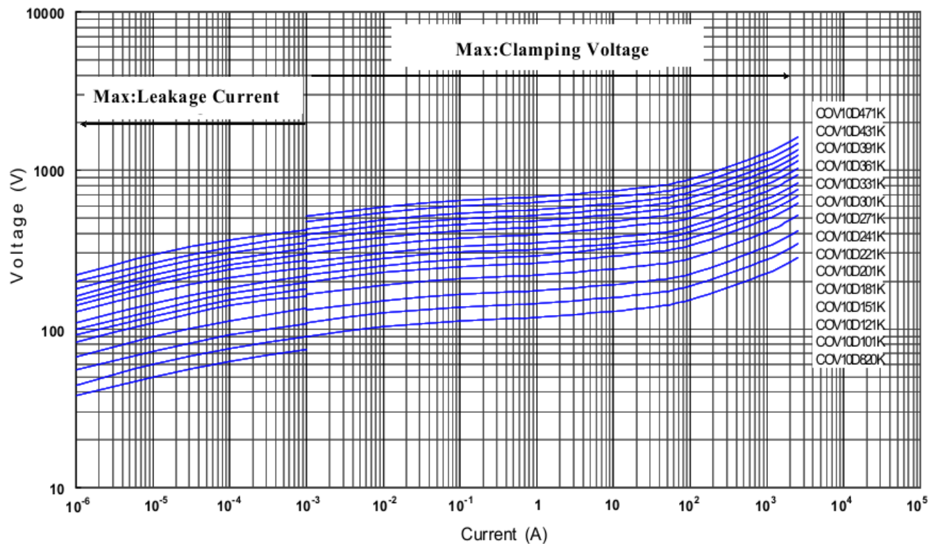
V-I Current (COV10D820K to COV10D471K)
