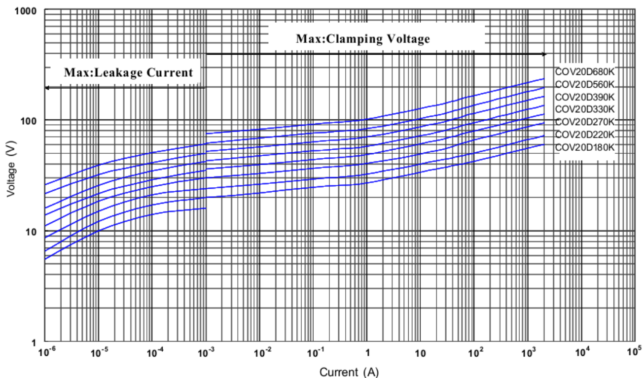
V - I (COV20D180K to COV20D680K)
