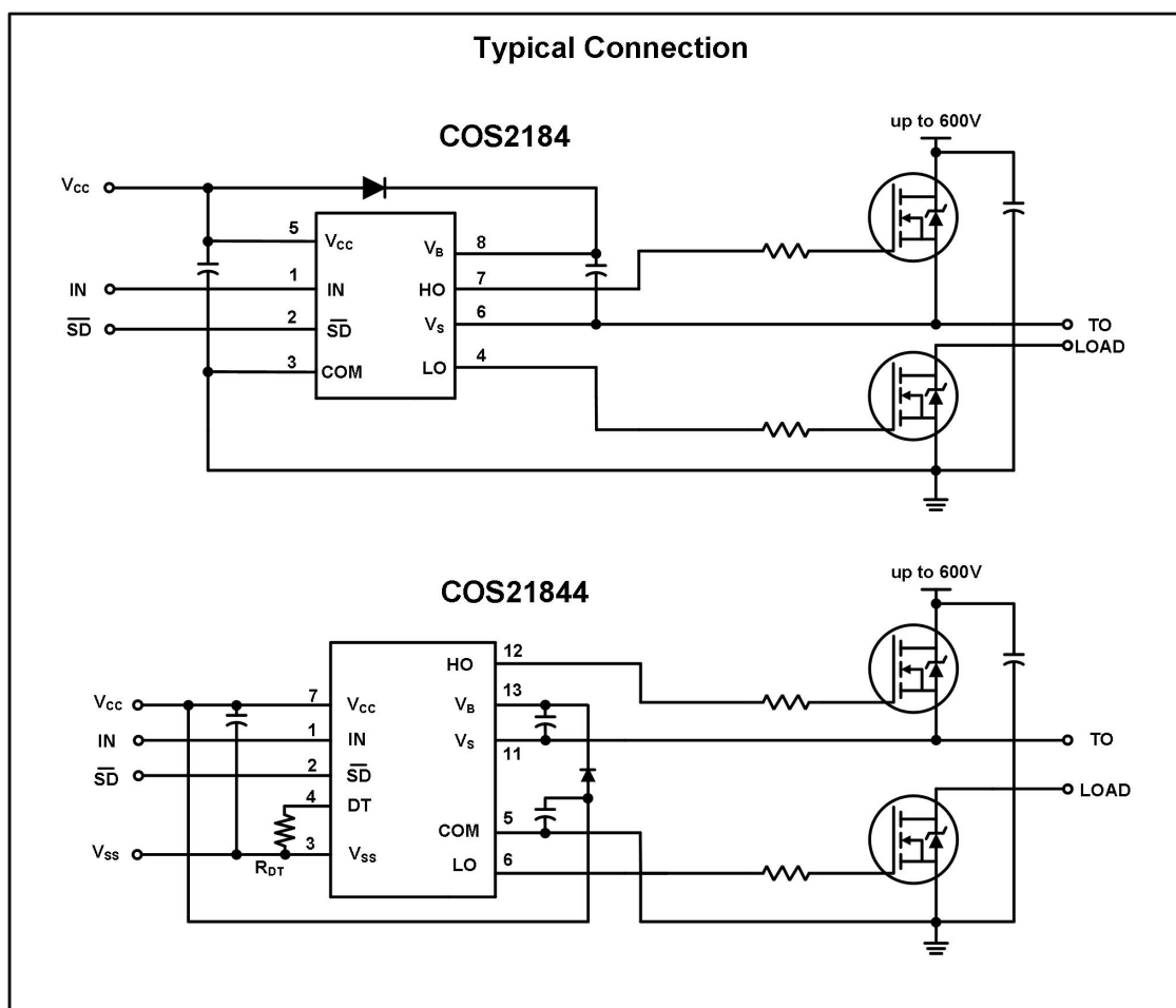
Figure 4. Typical Connection
