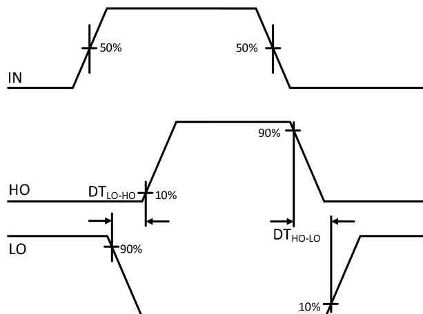
Figure 9. Deadtime Waveform Definitions
