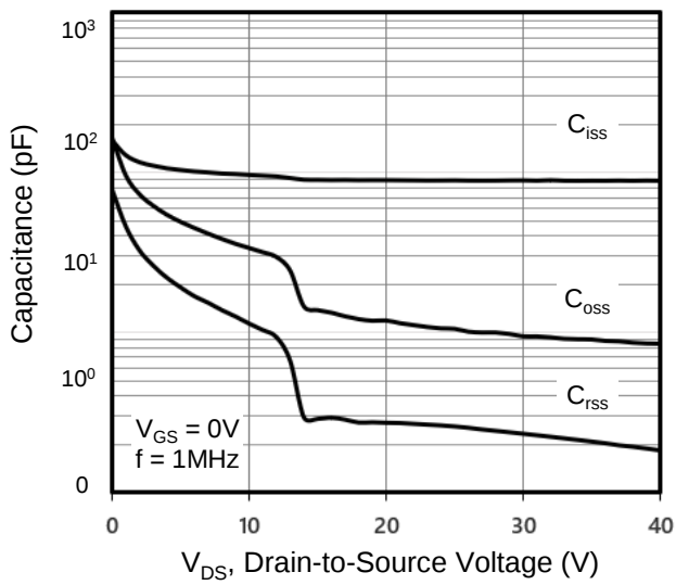
Figure 7. Capacitance
