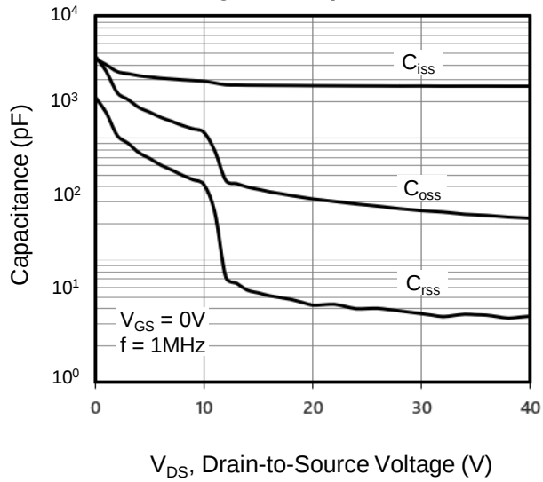
Figure 7. Capacitance
