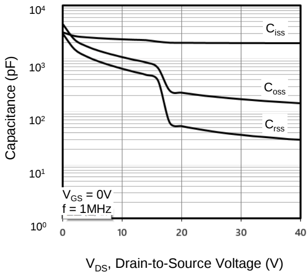
Figure 7. Capacitance
