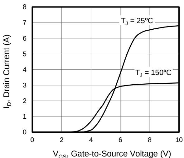
Figure 5. Transfer Characteristics
