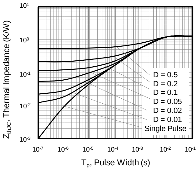
Figure 9. Transient Thermal Impedance TO-220, TO-251, TO-252
