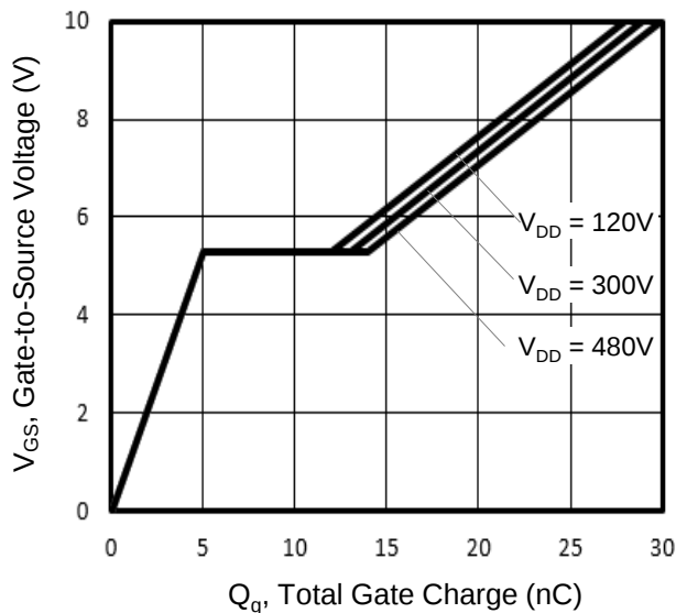
Figure 8. Gate Charge
