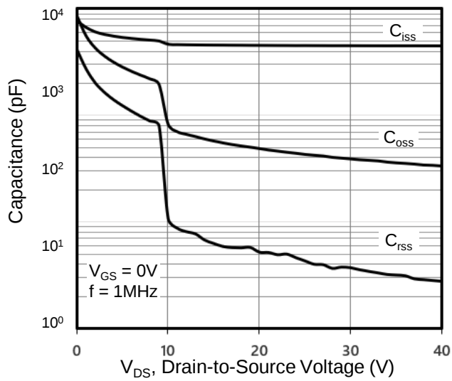
Figure 7. Capacitance
