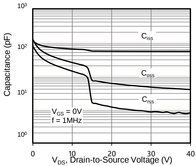
Figure 7. Capacitance
