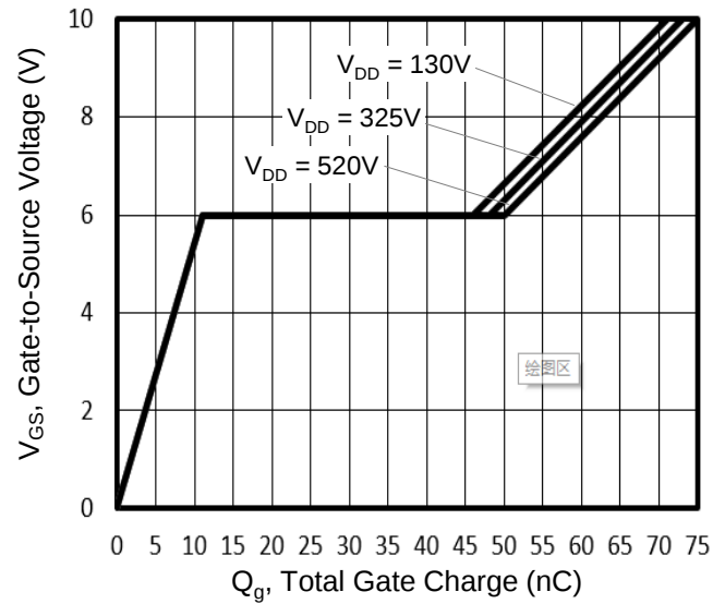
Figure 8. Gate Charge
