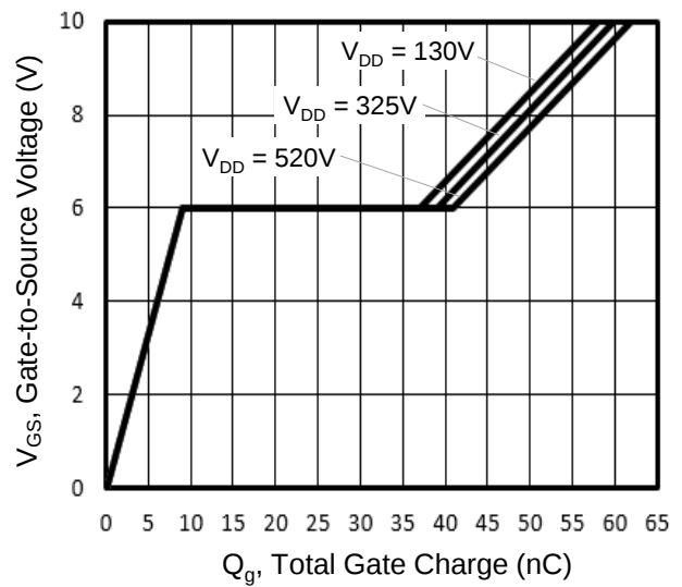
Figure 8. Gate Charge
