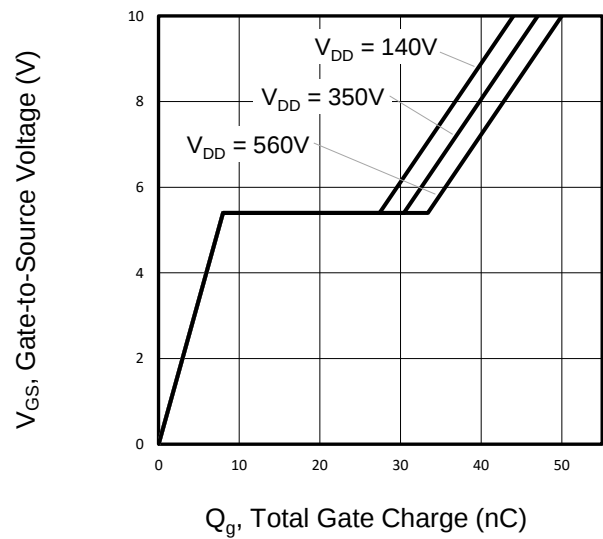
Figure 8. Gate Charge
