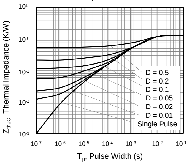
Figure 9. Transient Thermal Impedance TO-262, TO-220
