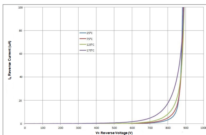
Fig. 2 Reverse Characteristics
