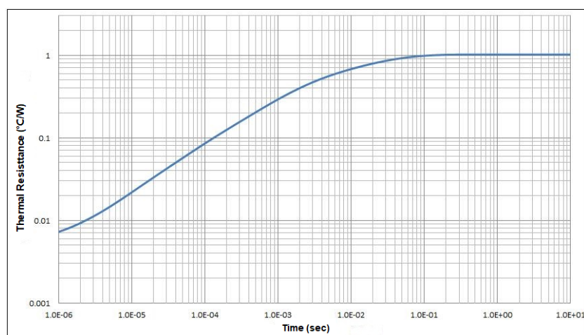
Fig. 5 Thermal characteristic curve
