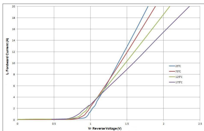
Fig. 1 Forward Characteristics
