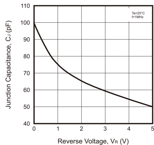
Fig.4 - Capacitance Characteristics
