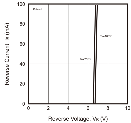
Fig.2 - Reverse Characteristic
