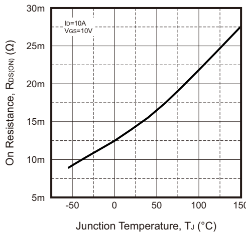
Fig.5 - Drain-Source On-State Resistance
