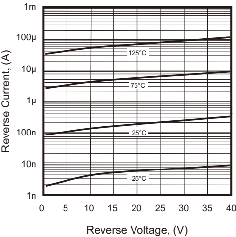
Fig.2 - Reverse Characteristics
