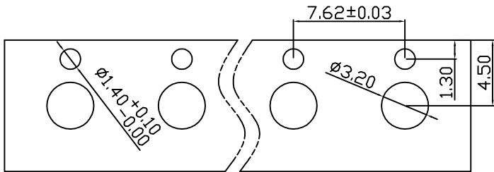
PCB LAYOUT
