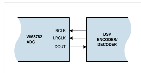
Figure 7 Slave Mode
