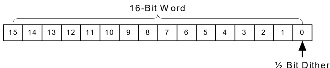
Figure 9. ADC 16-Bit Auto-Dither
