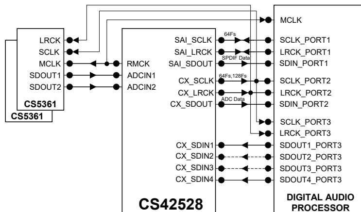
Figure 18. OLM Configuration #3
