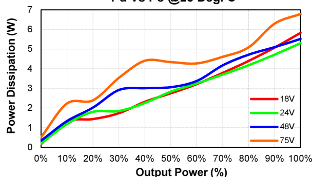
ECLB60W-48D12 Pd Vs Po @25 Deg. C
