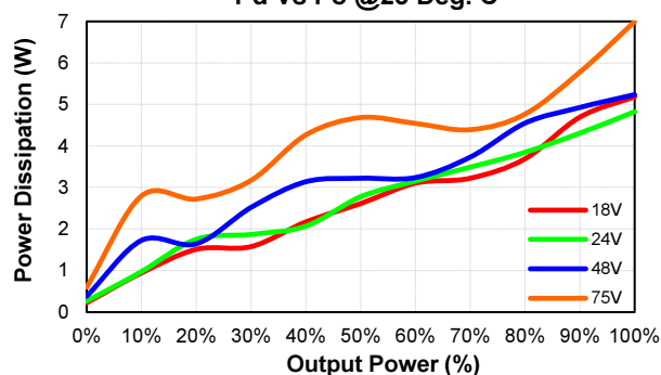
ECLB60W-48D15 Pd Vs Po @25 Deg. C
