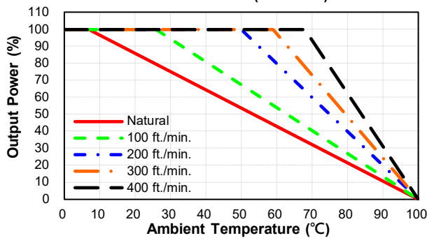
CQB100-110S3V3 Derating Curve without Heatsink (Vin=110V)
