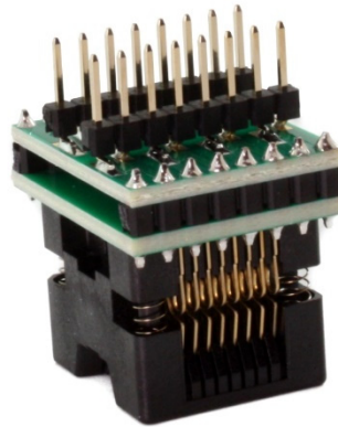
Image 2: Bottom View of Socket Adapter
