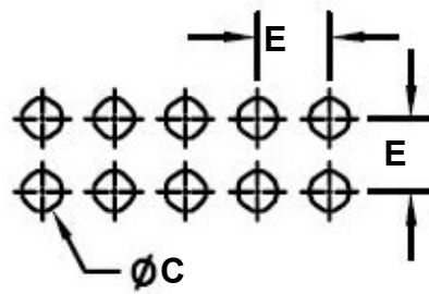
Recommended PCB Hole Layout for MPH-ETD pair
