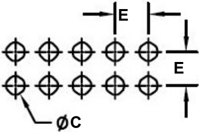
Recommended PCB Hole Layout for MPH-ETD pair
