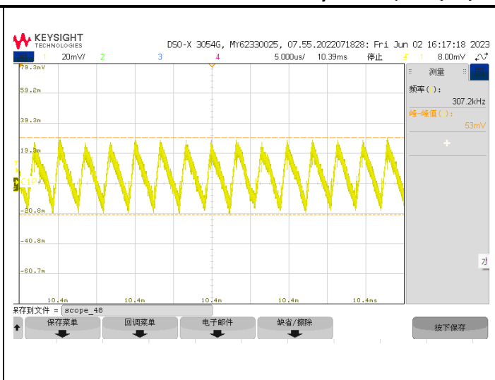
VINP=5V, V ISO =3.7V, I SO =300mA, V ISO 纹波电压峰峰值
