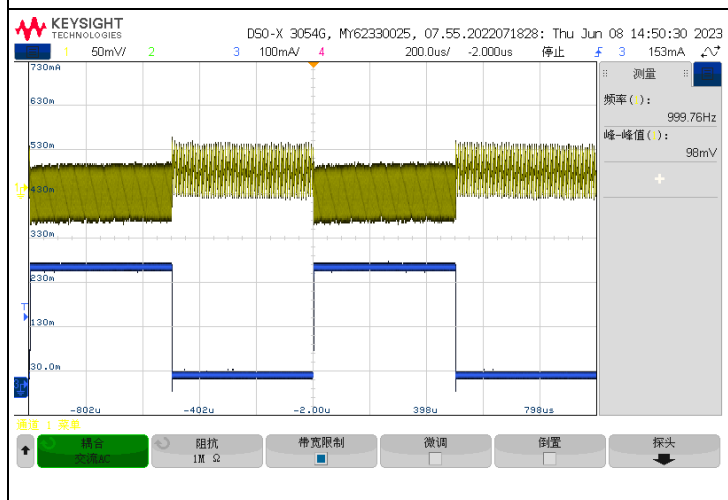
VINP =5V, V ISO =5V, 动态负载电流: 30mA/270mA
