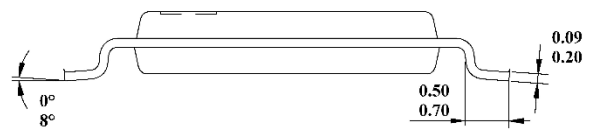
LEFT VIEW
