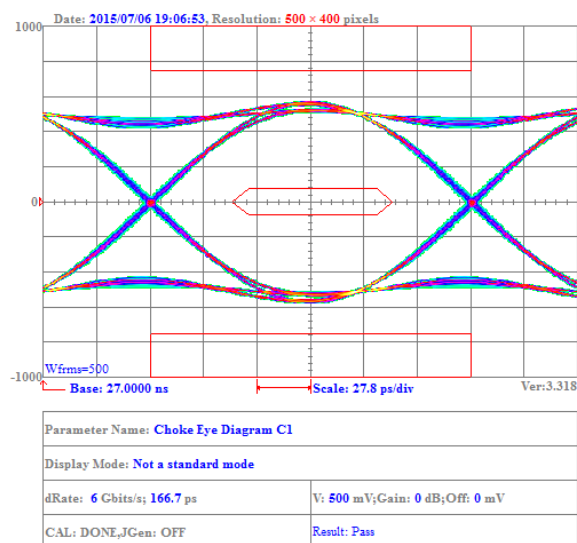
Eye Diagram For HDMI2.0 Testing:
