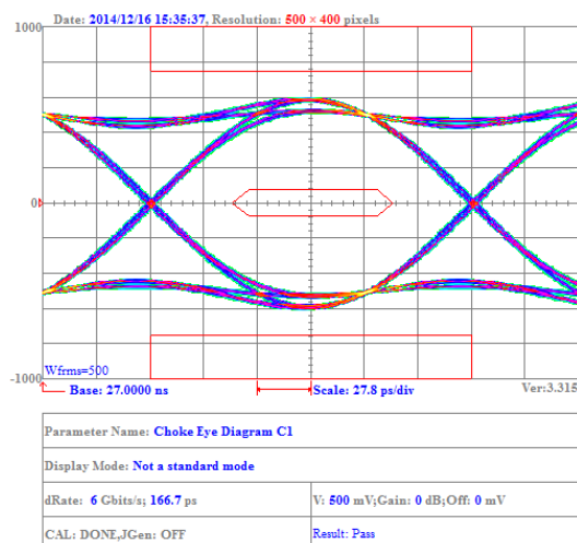
Eye Diagram For HDMI2.0 Testing:
