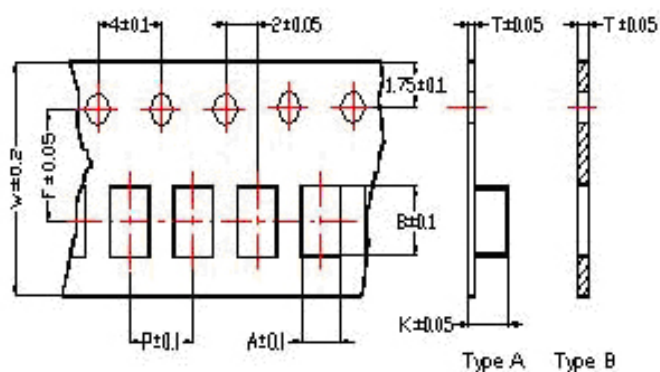
Tape Dimensions
