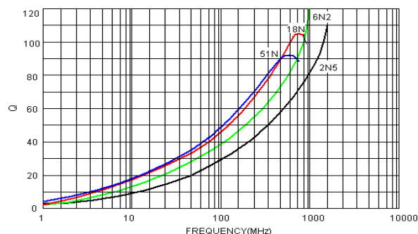
Typical Q vs. Frequency
