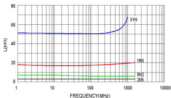
Typical L vs. Frequency
