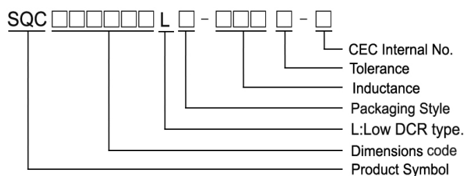
SQC322520 & SQC322520LT
