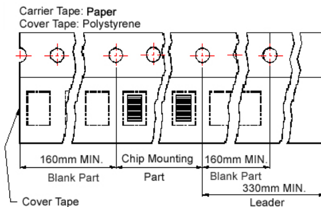
Tape Material
