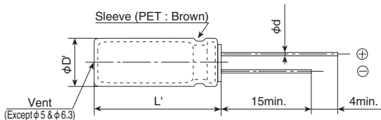
(φ 5 to φ 10) (φ 12.5 to φ 18) Gas escape end seal
