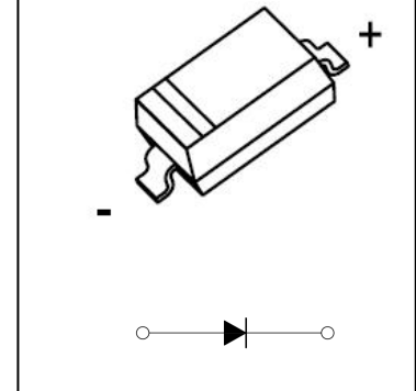
SOD-123
